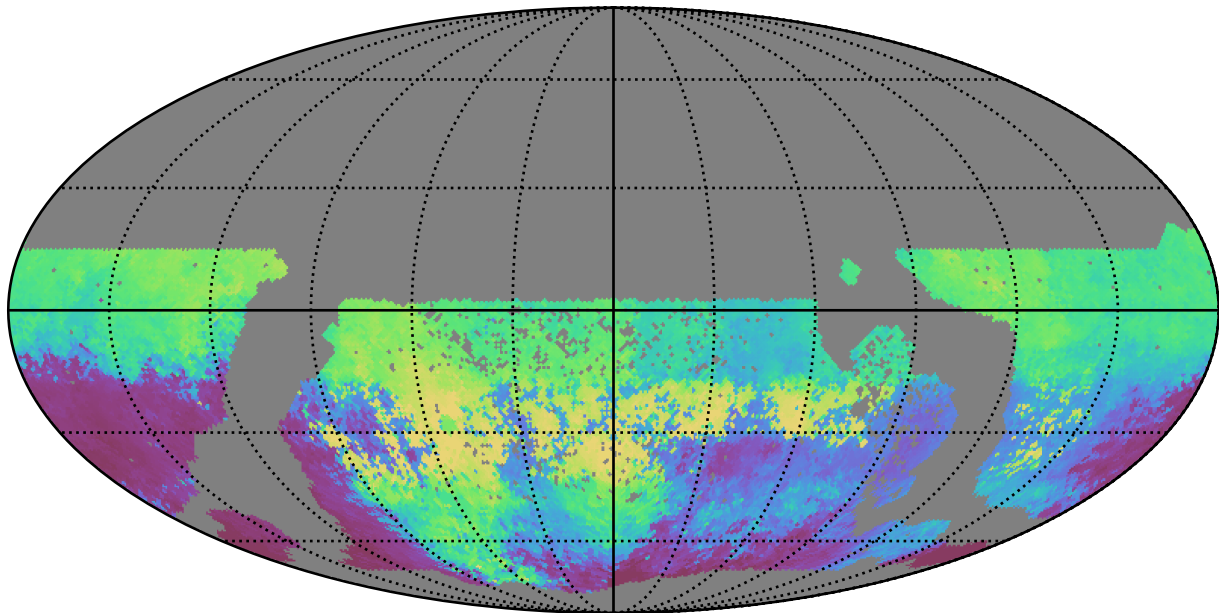
all_long_v3.4_10yrs WFD g band: Median HA
