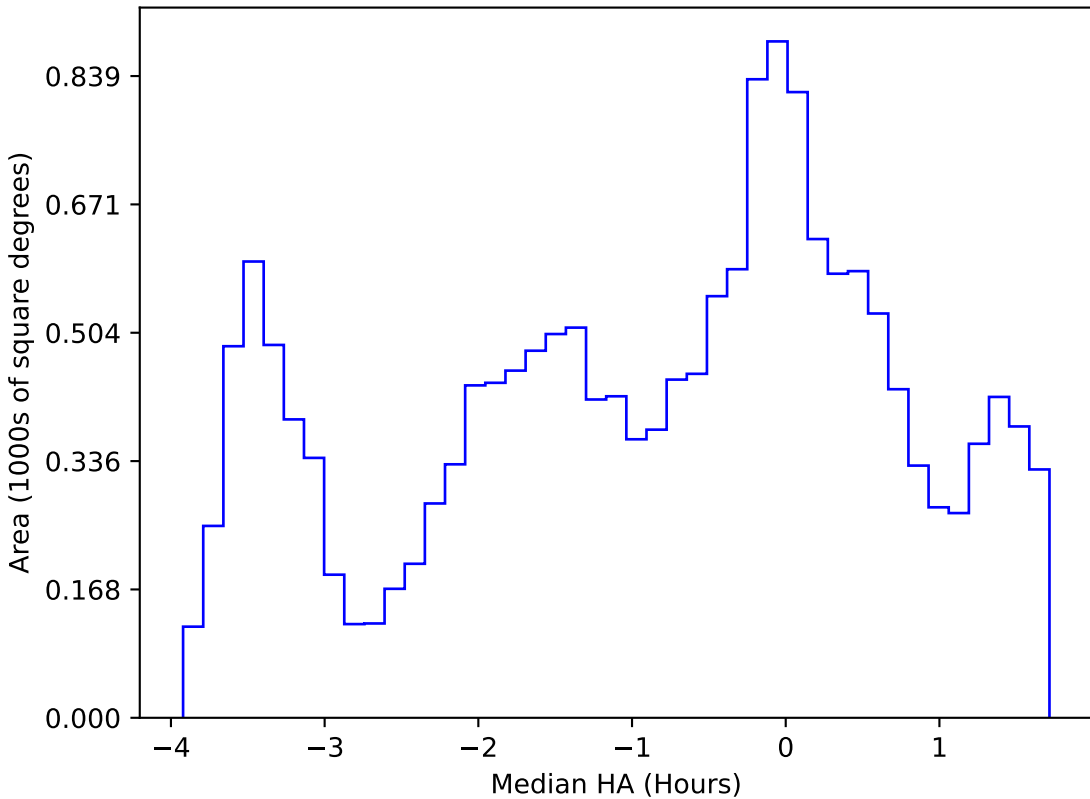
all_long_v3.4_10yrs WFD g band: Median HA
