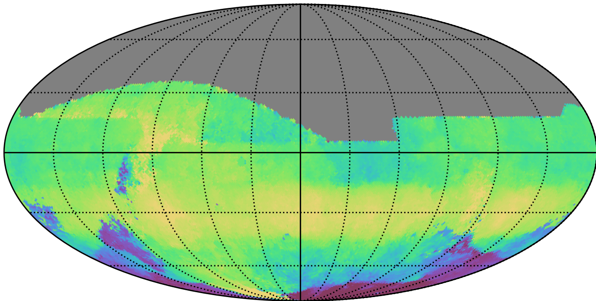
all_long_v3.4_10yrs All sky z band: Median HA
