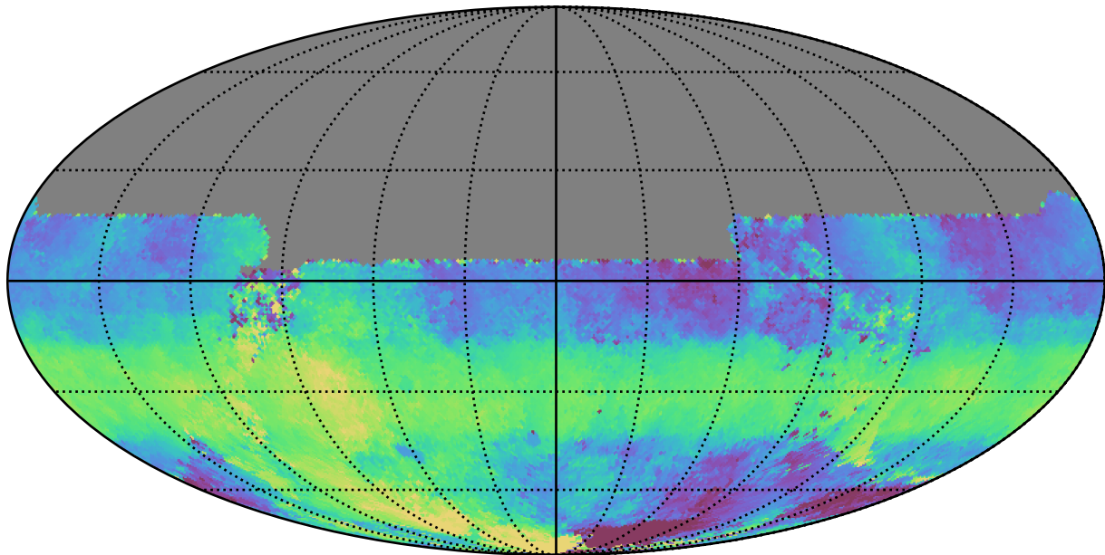
all_long_v3.4_10yrs All sky u band: Median HA
