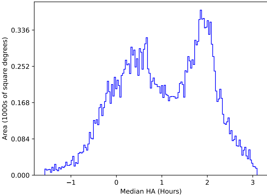
all_long_v3.4_10yrs All sky u band: Median HA
