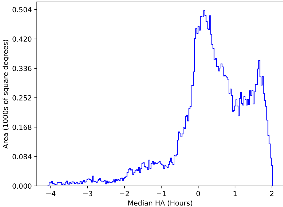
all_long_v3.4_10yrs All sky r band: Median HA
