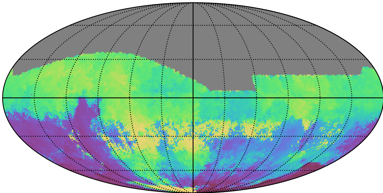
all_long_v3.4_10yrs All sky g band: Median HA
