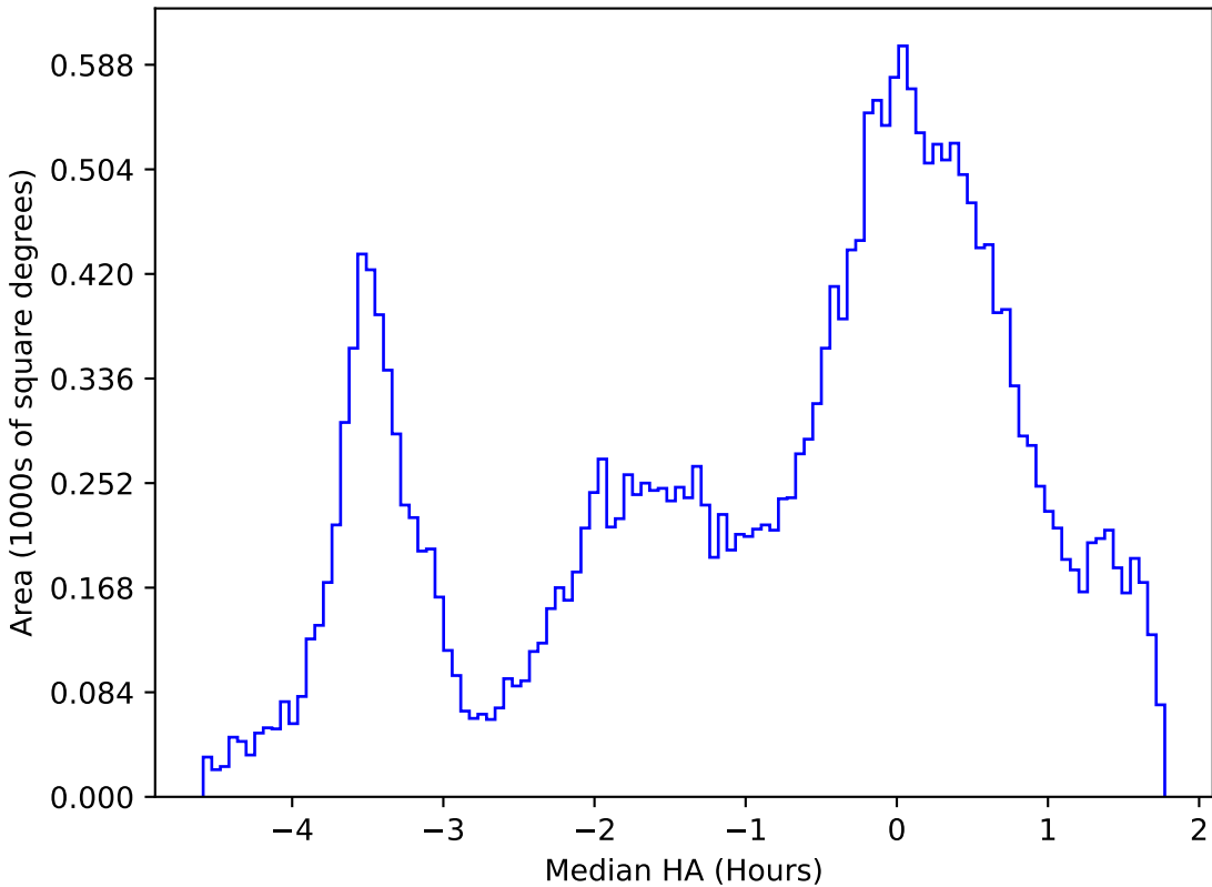
all_long_v3.4_10yrs All sky g band: Median HA
