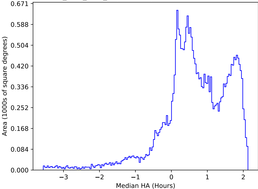
all_long_v3.4_10yrs All sky all bands: Median HA
