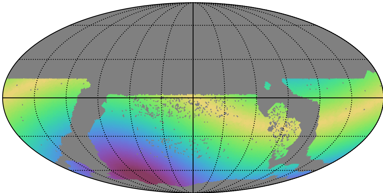
all_long_v3.4_10yrs WFD z band: Max solarElong
