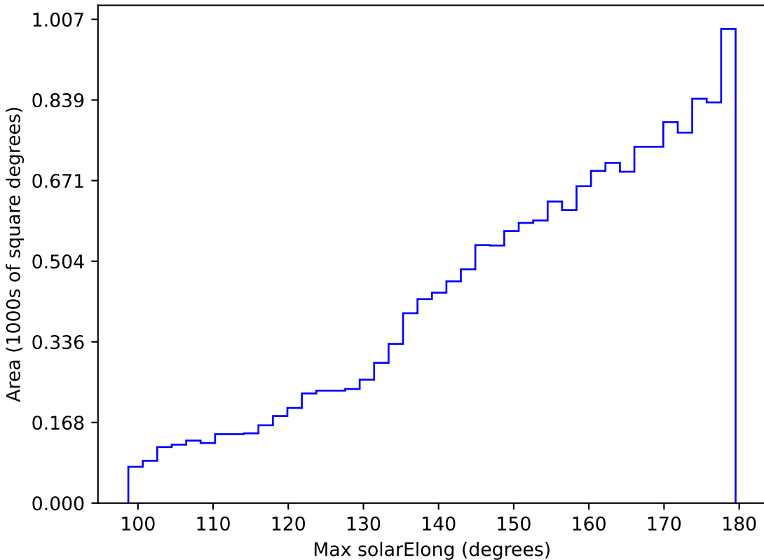
all_long_v3.4_10yrs WFD z band: Max solarElong
