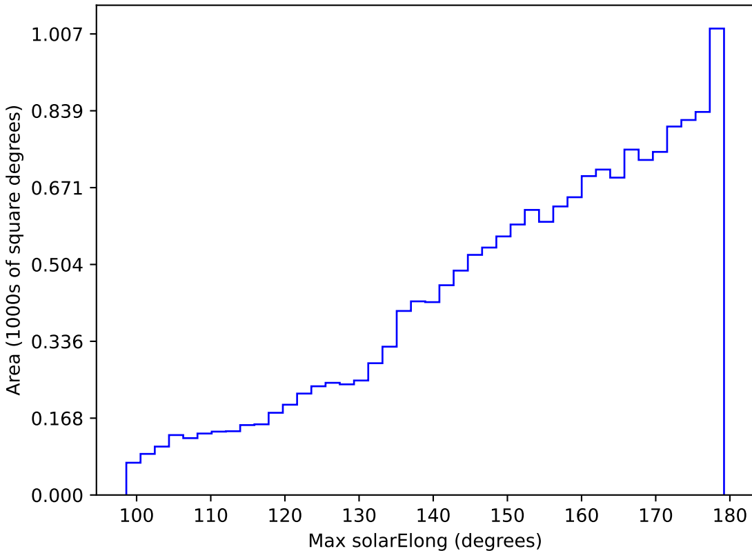
all_long_v3.4_10yrs WFD y band: Max solarElong
