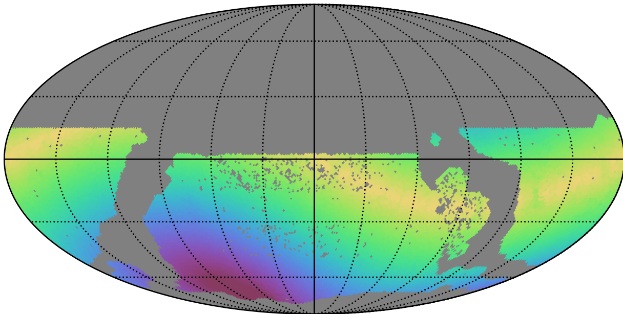
all_long_v3.4_10yrs WFD u band: Max solarElong
