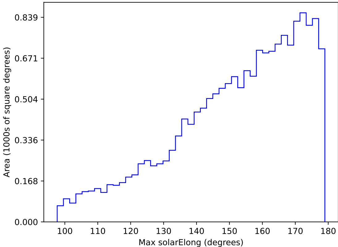
all_long_v3.4_10yrs WFD u band: Max solarElong
