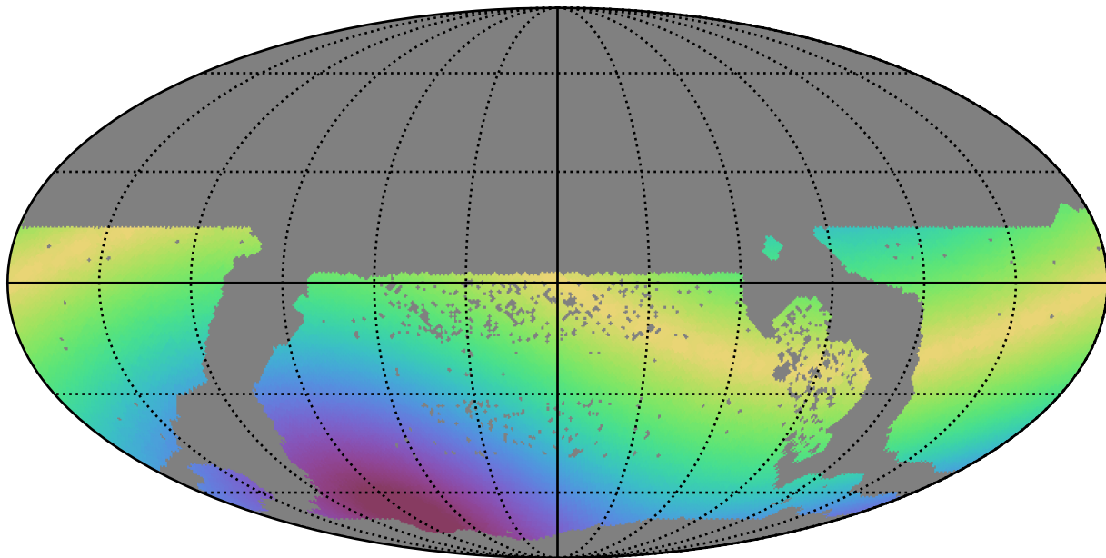
all_long_v3.4_10yrs WFD i band: Max solarElong
