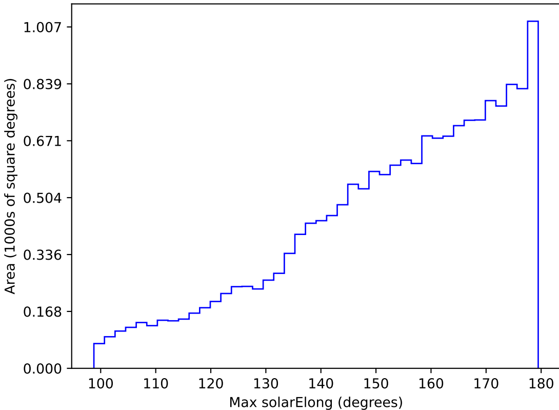
all_long_v3.4_10yrs WFD i band: Max solarElong
