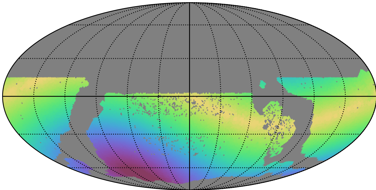
all_long_v3.4_10yrs WFD g band: Max solarElong
