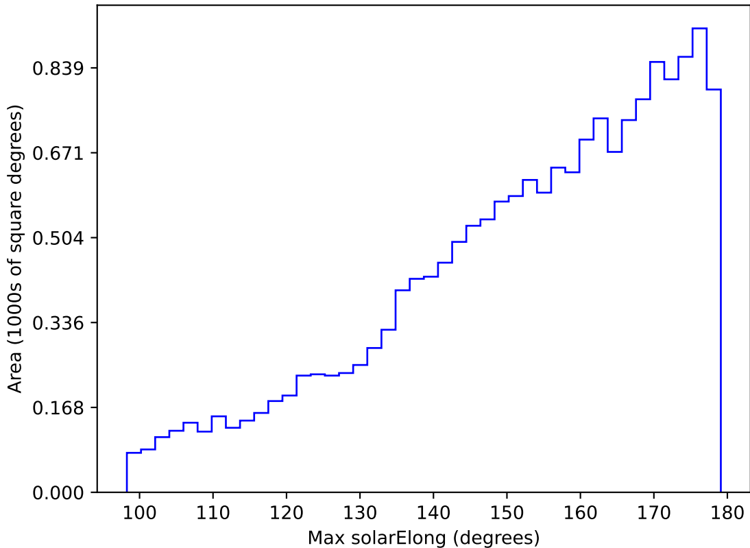
all_long_v3.4_10yrs WFD g band: Max solarElong
