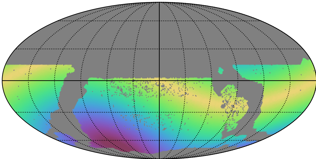
all_long_v3.4_10yrs WFD all bands: Max solarElong
