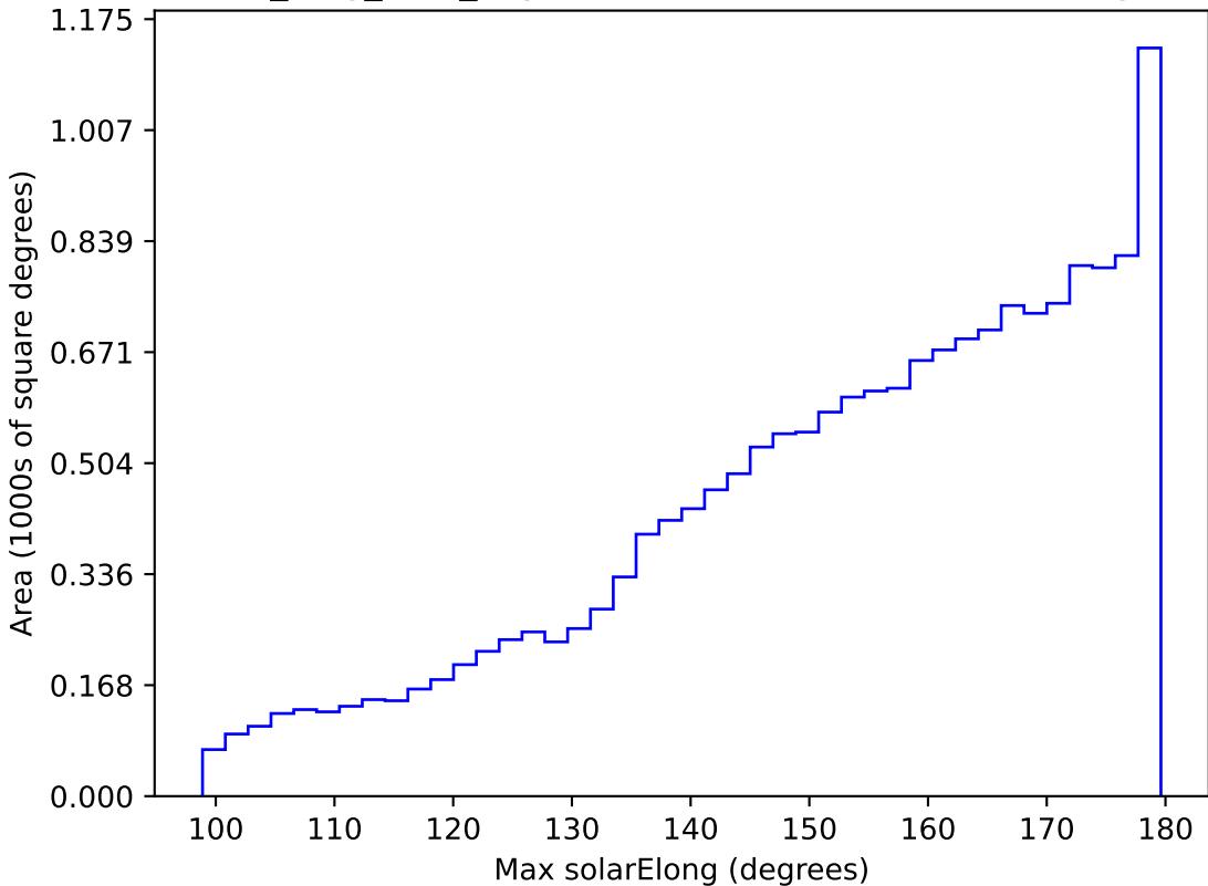
all_long_v3.4_10yrs WFD all bands: Max solarElong
