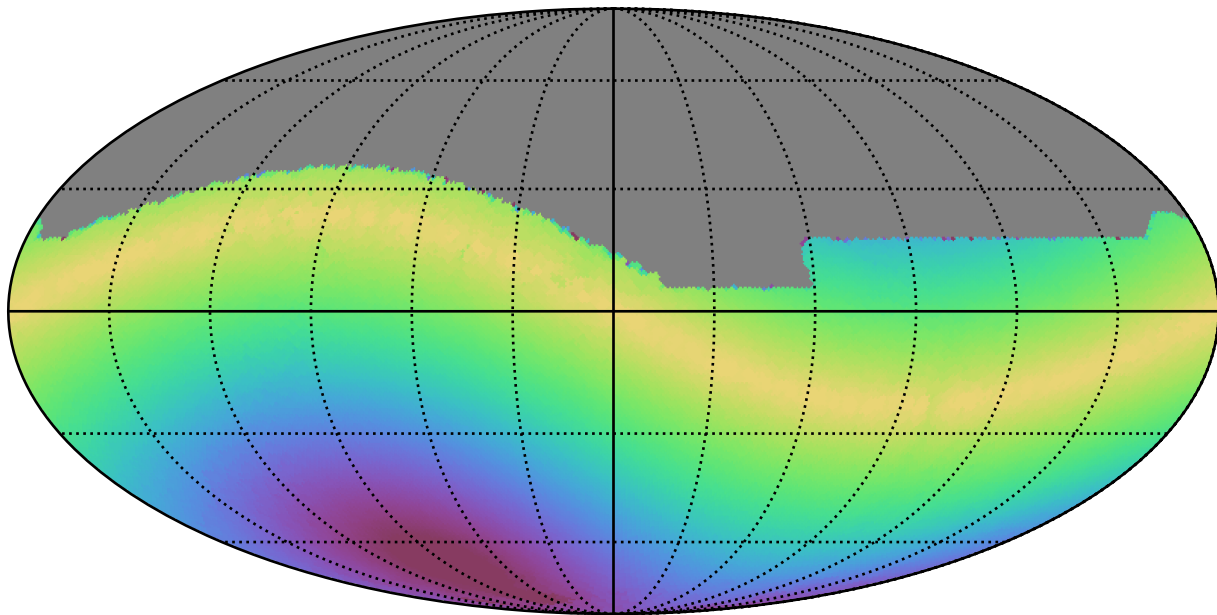
all_long_v3.4_10yrs All sky r band: Max solarElong
