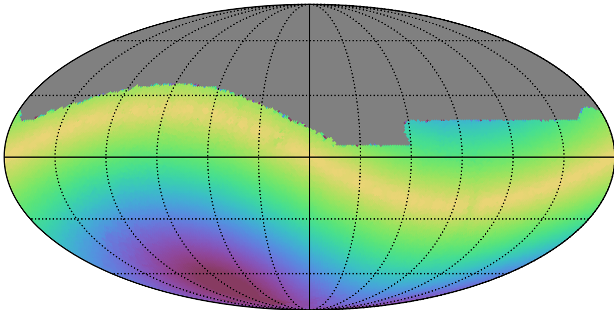
all_long_v3.4_10yrs All sky i band: Max solarElong
