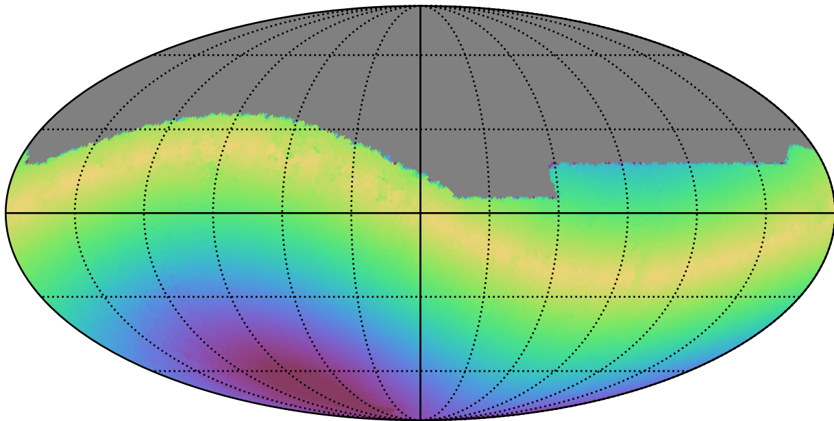
all_long_v3.4_10yrs All sky g band: Max solarElong
