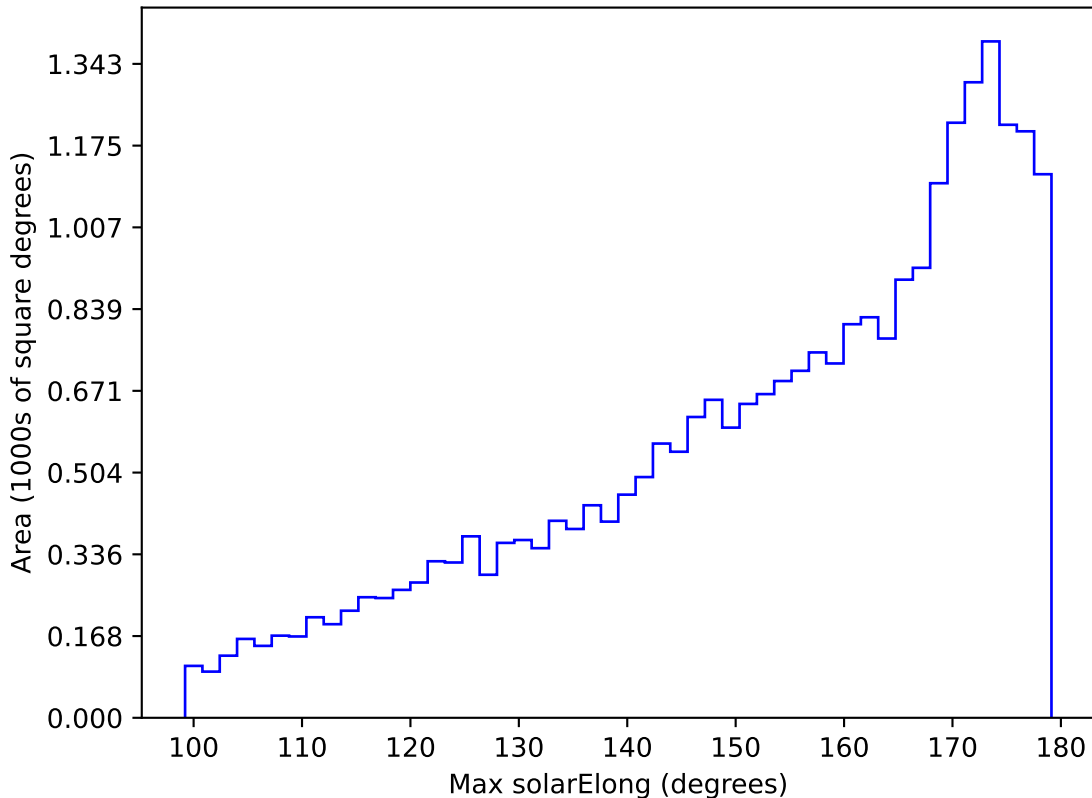
all_long_v3.4_10yrs All sky g band: Max solarElong
