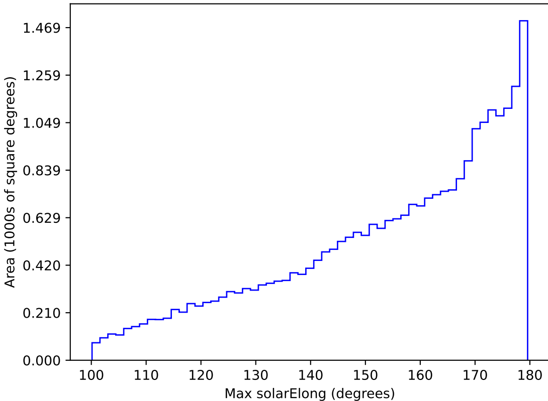
all_long_v3.4_10yrs All sky all bands: Max solarElong
