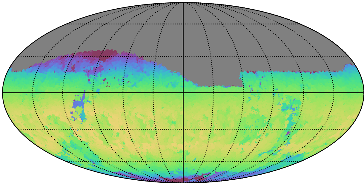
all_long_v3.4_10yrs Yr 1 z band: Max skyBrightness
