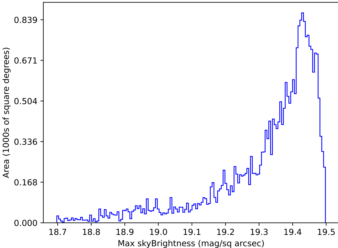
all_long_v3.4_10yrs Yr 1 z band: Max skyBrightness
