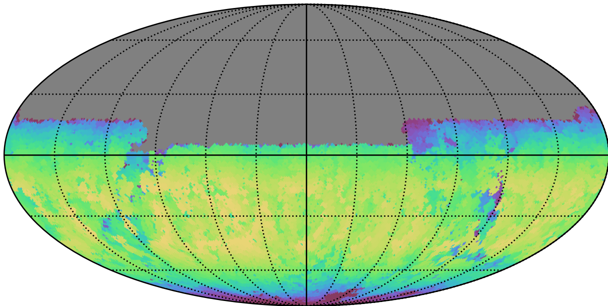
all_long_v3.4_10yrs Yr 1 y band: Max skyBrightness
