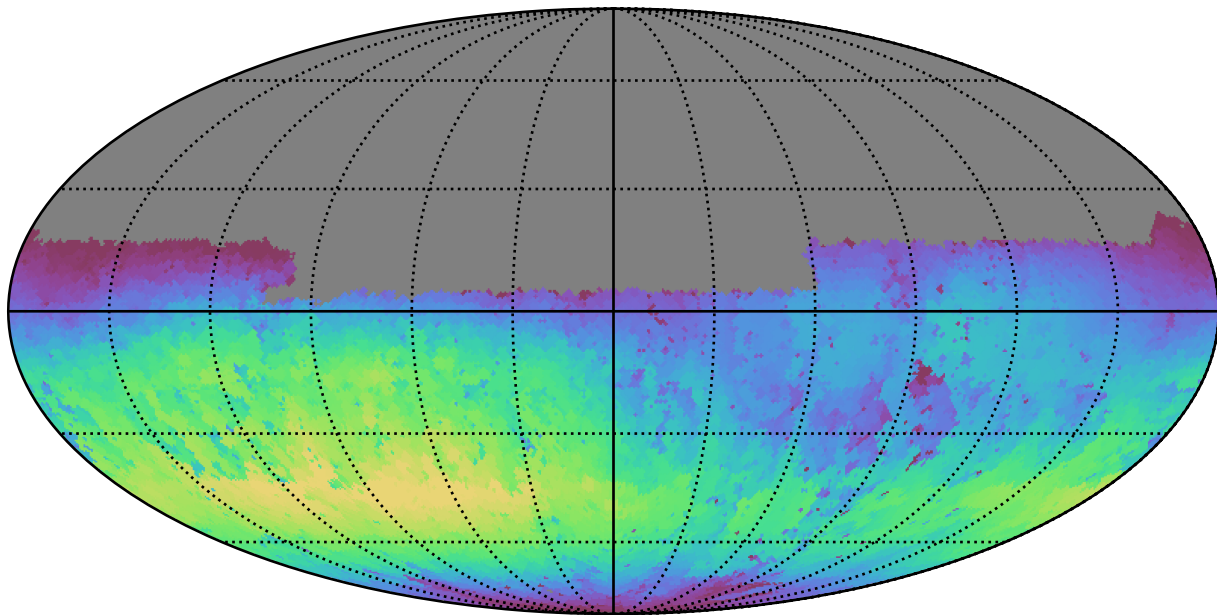
all_long_v3.4_10yrs Yr 1 u band: Max skyBrightness
