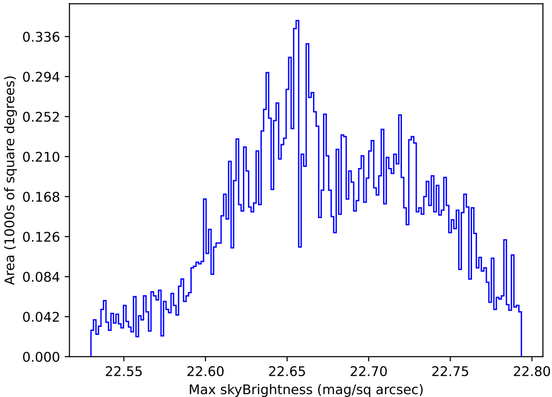
all_long_v3.4_10yrs Yr 1 u band: Max skyBrightness
