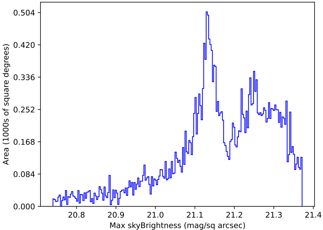
all_long_v3.4_10yrs Yr 1 r band: Max skyBrightness
