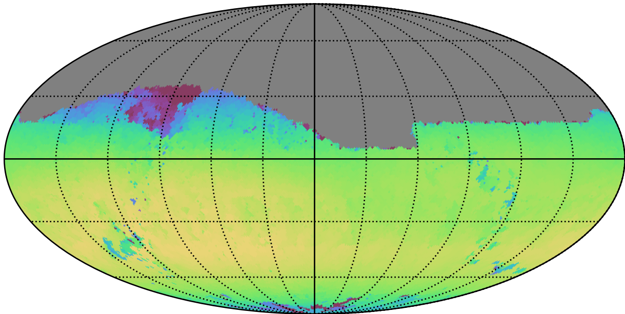
all_long_v3.4_10yrs Yr 1 i band: Max skyBrightness
