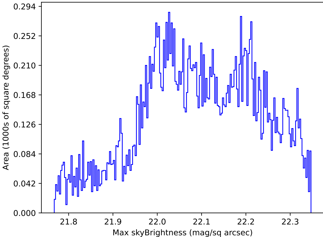
all_long_v3.4_10yrs Yr 1 g band: Max skyBrightness
