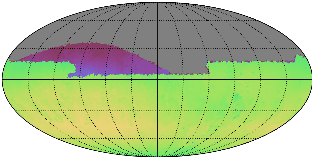
all_long_v3.4_10yrs Yr 1 all bands: Max skyBrightness
