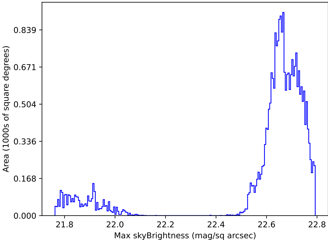
all_long_v3.4_10yrs Yr 1 all bands: Max skyBrightness
