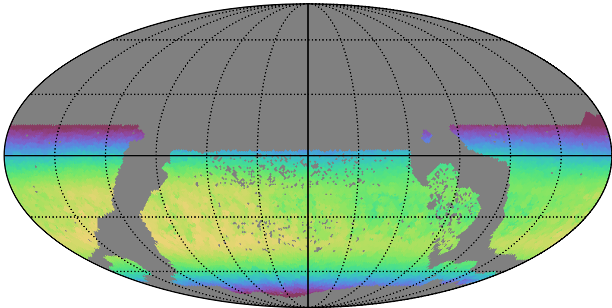
all_long_v3.4_10yrs WFD z band: Max skyBrightness
