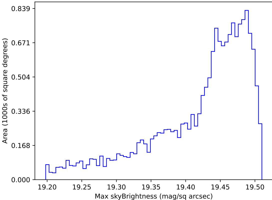
all_long_v3.4_10yrs WFD z band: Max skyBrightness
