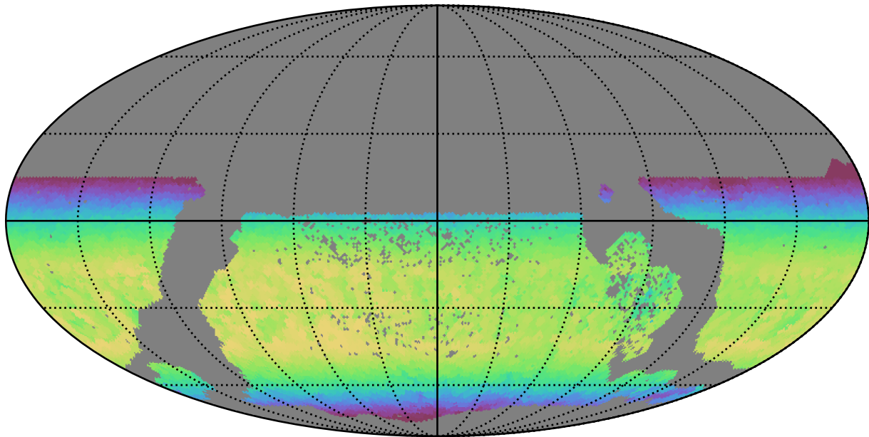
all_long_v3.4_10yrs WFD y band: Max skyBrightness
