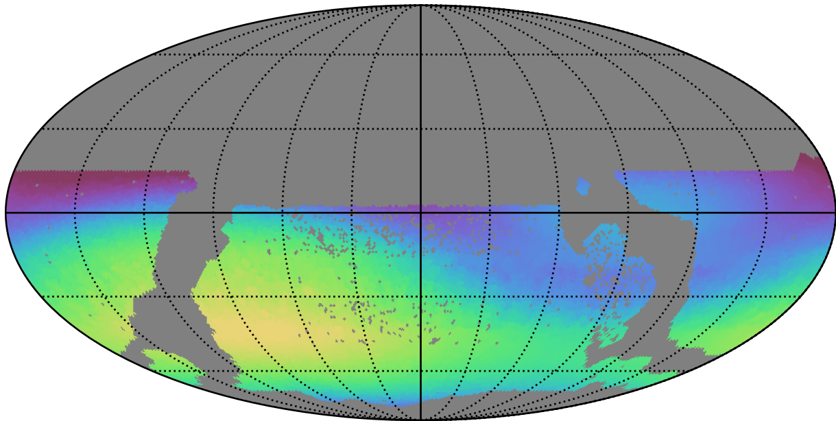
all_long_v3.4_10yrs WFD r band: Max skyBrightness
