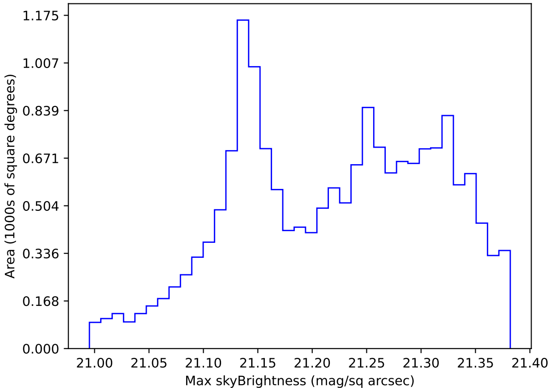
all_long_v3.4_10yrs WFD r band: Max skyBrightness
