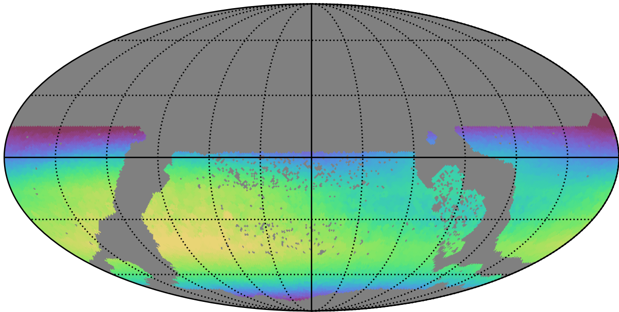
all_long_v3.4_10yrs WFD i band: Max skyBrightness
