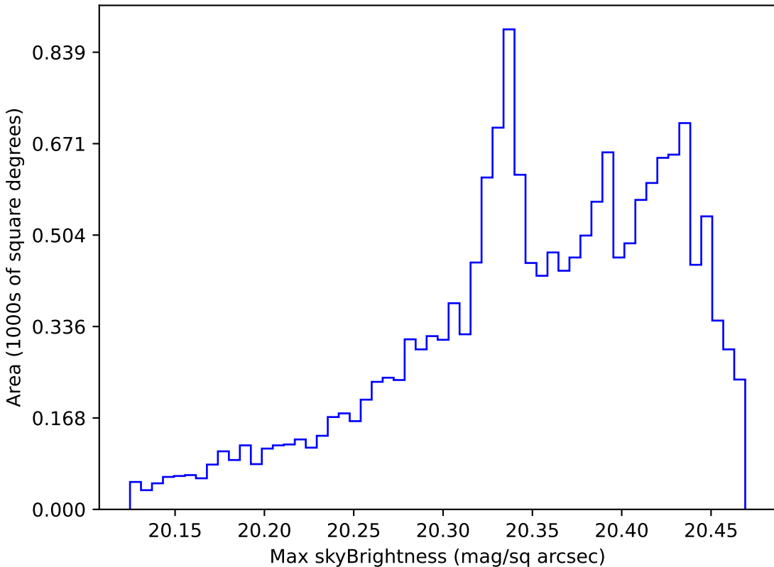
all_long_v3.4_10yrs WFD i band: Max skyBrightness
