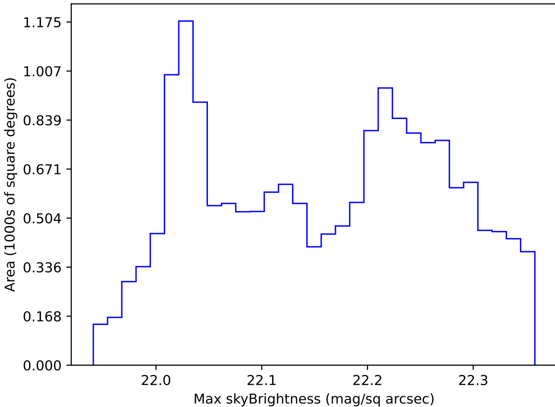
all_long_v3.4_10yrs WFD g band: Max skyBrightness
