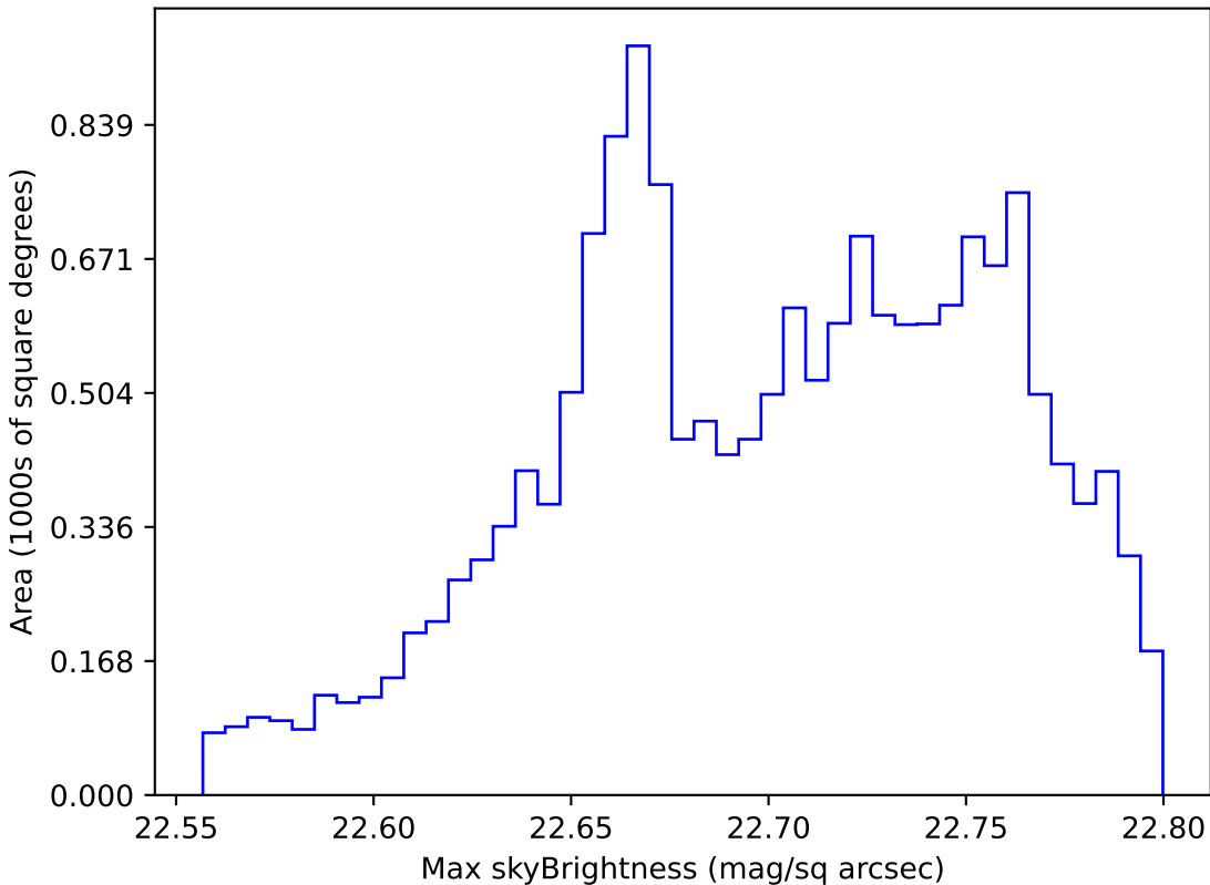
all_long_v3.4_10yrs WFD all bands: Max skyBrightness
