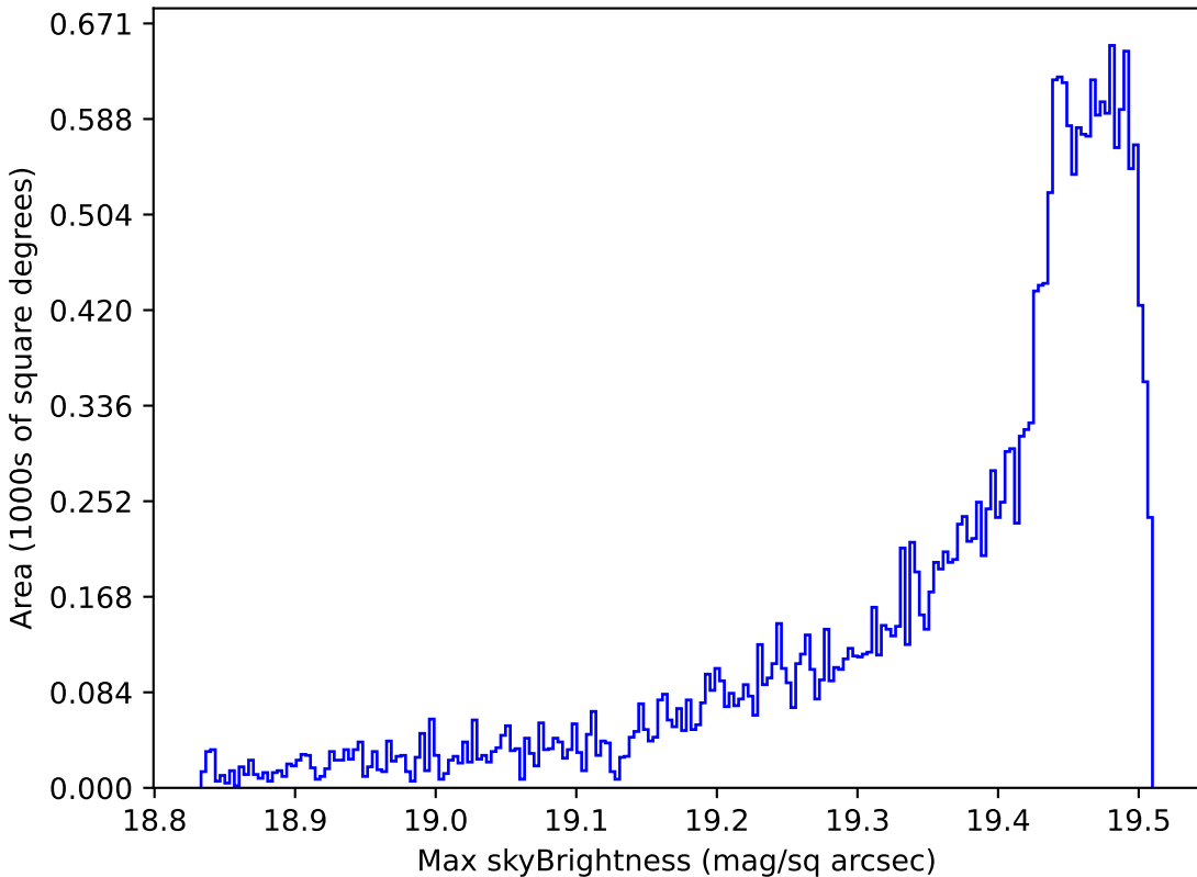
all_long_v3.4_10yrs All sky z band: Max skyBrightness
