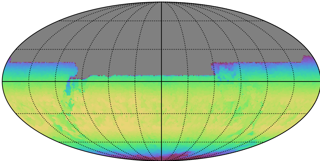
all_long_v3.4_10yrs All sky y band: Max skyBrightness
