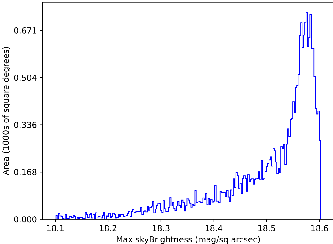
all_long_v3.4_10yrs All sky y band: Max skyBrightness
