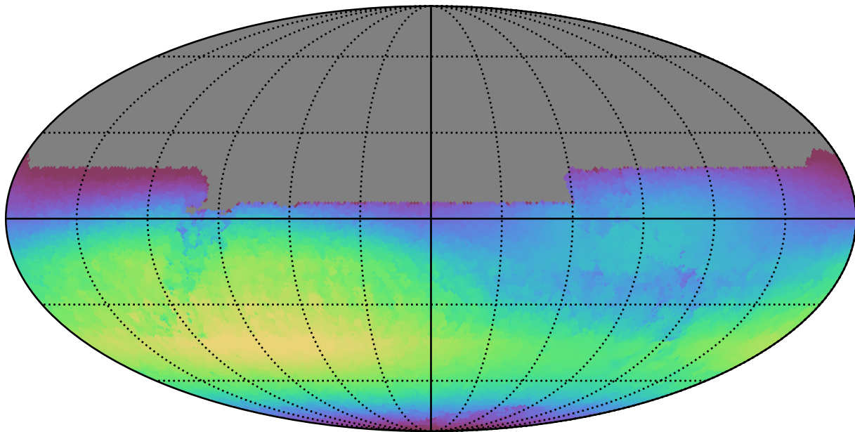
all_long_v3.4_10yrs All sky u band: Max skyBrightness
