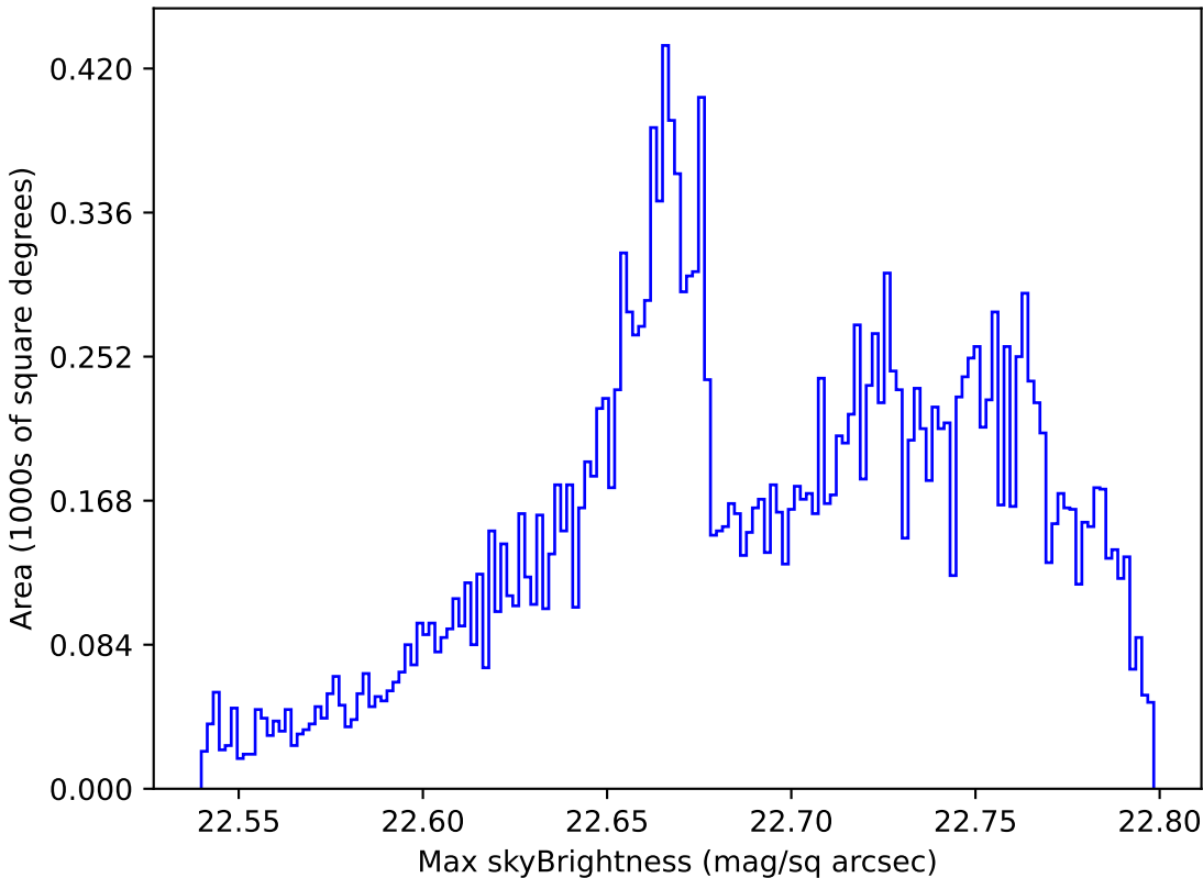
all_long_v3.4_10yrs All sky u band: Max skyBrightness
