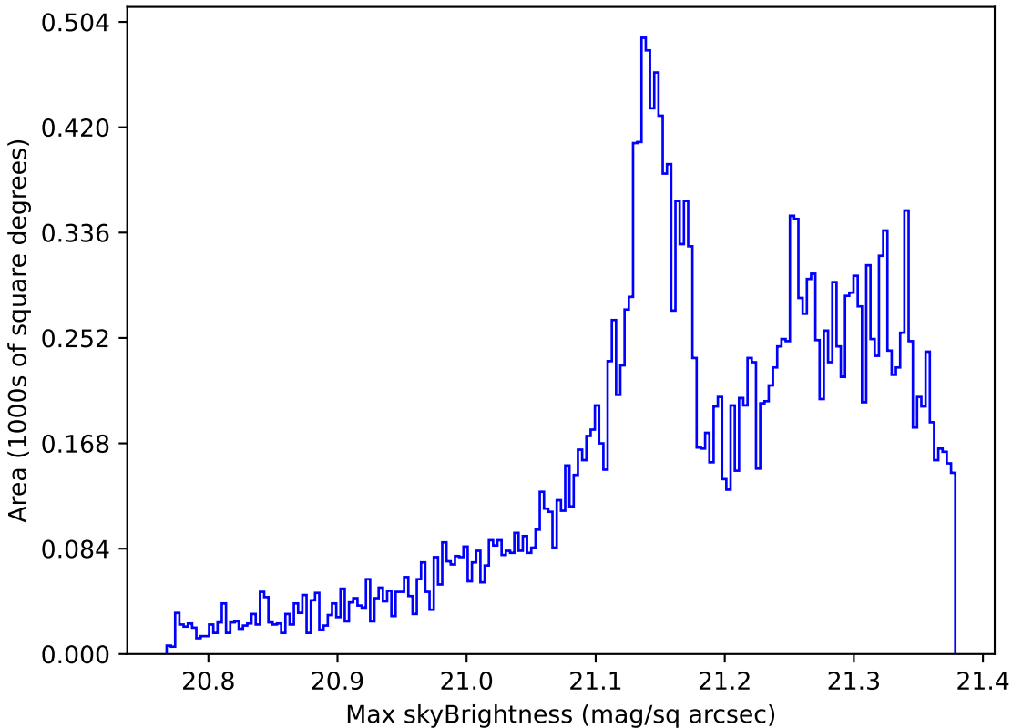
all_long_v3.4_10yrs All sky r band: Max skyBrightness
